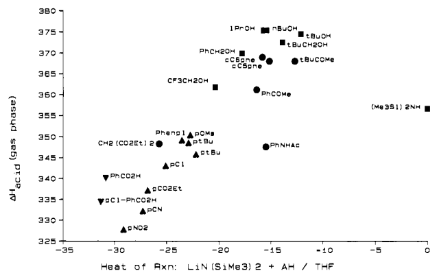
Figure 3. Gas-phase anion proton affinity ( \Delta H_{\text{acid}} ) vs enthalpy of solution-phase proton transfer from various acids to lithiated hexamethyldisilazide ( 2b ) in THF solvent, in kcal/mol: (▲) phenols, (▼) benzoic acids, (●) ketones and esters, (■) "localized" OH, NH acids.
